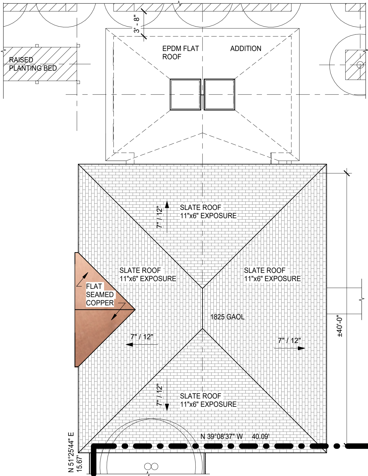
1 Site Plan 1/8" = 1'-0"
