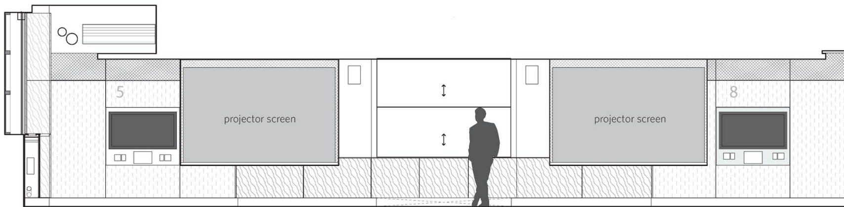
LECTURE CLASSROOM - TEACHING WALL ELEVATION
