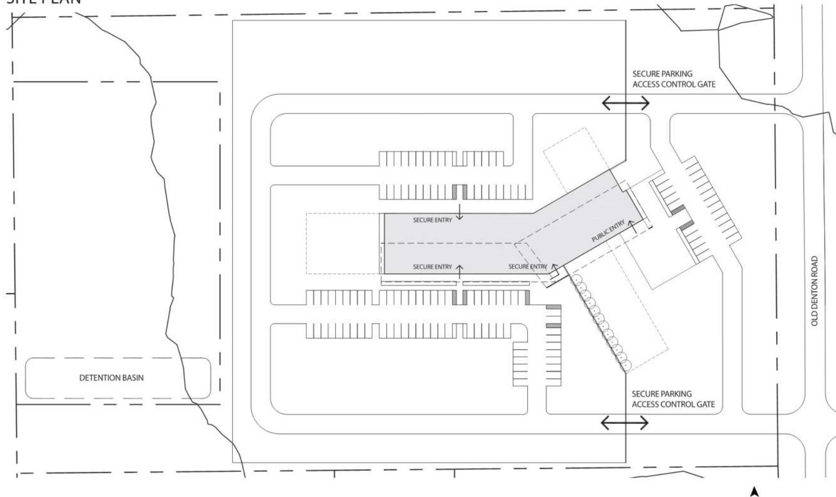
SITE PLAN
