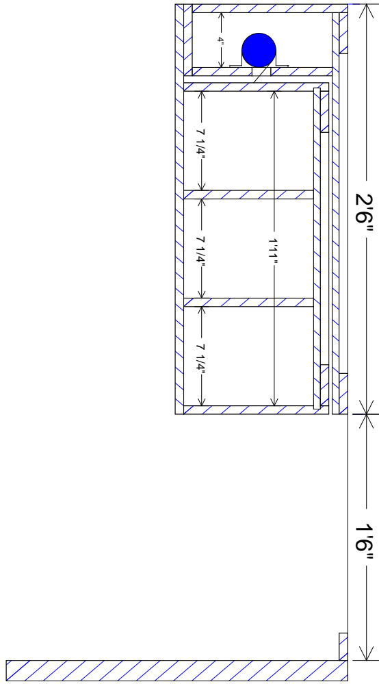
Section Through - Side View - Closed
