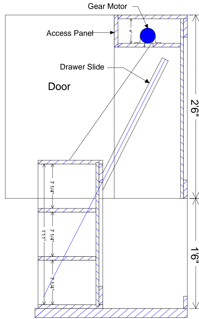
Section Through - Side View - Deployed
